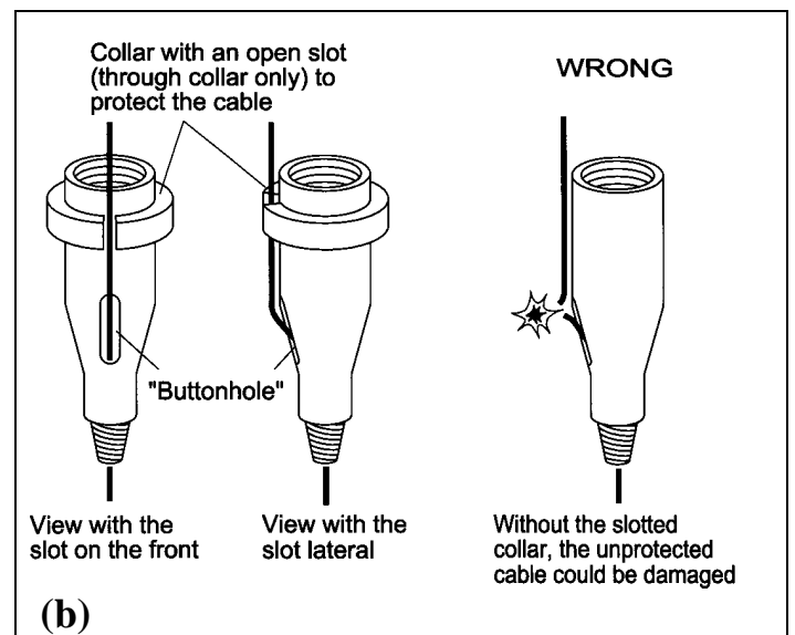
Fig. 9. (a) Possible exits of the cable from the rods (b) Intermediate slotted adaptor joining the upper push rods to the torpedo-like bottom assembly of blade and rods
