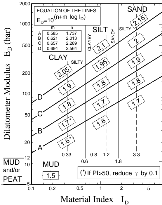
Fig. 16. Chart for estimating soil type and unit weight \gamma (normalized to \gamma_w = \gamma water) - Marchetti & Crapps 1981 - (1 bar = 100 kPa)
