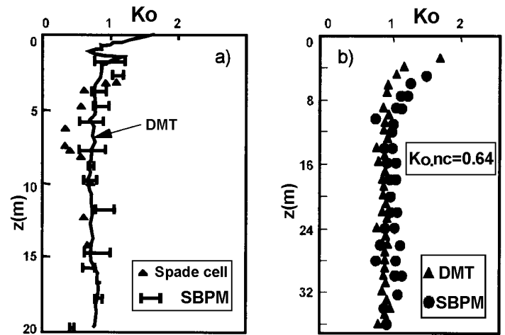
Fig. 19. K_0 from DMT vs K_0 by other methods at two clay research sites (Aversa 1997)
